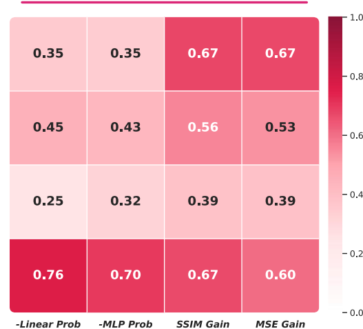
Spearman Correlation ( \rho )
