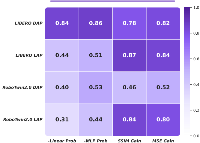
Pearson Correlation (r)
