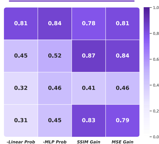
Pearson Correlation (r)
